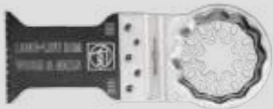
E-CUT LONG LIFE BLADE PART NUMBER: 63502160290
