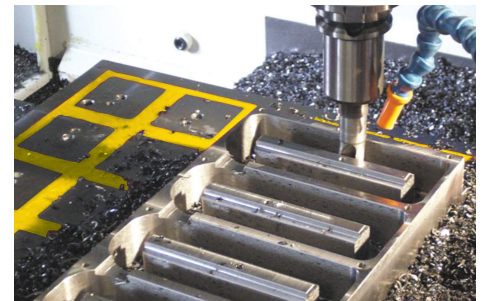
Machining mold cavities
