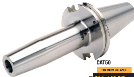
CAT40 PREMIUM BALANCE G2.5 at 30,000rpm CERTIFICATE INCLUDED
