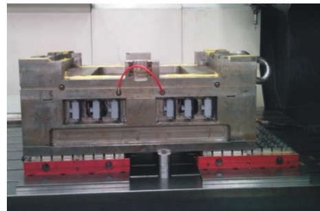
Machining injection mold application
